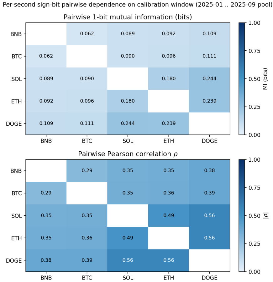
Figure 4.10: Experiment 4 – calibration-window mutual information matrix.
