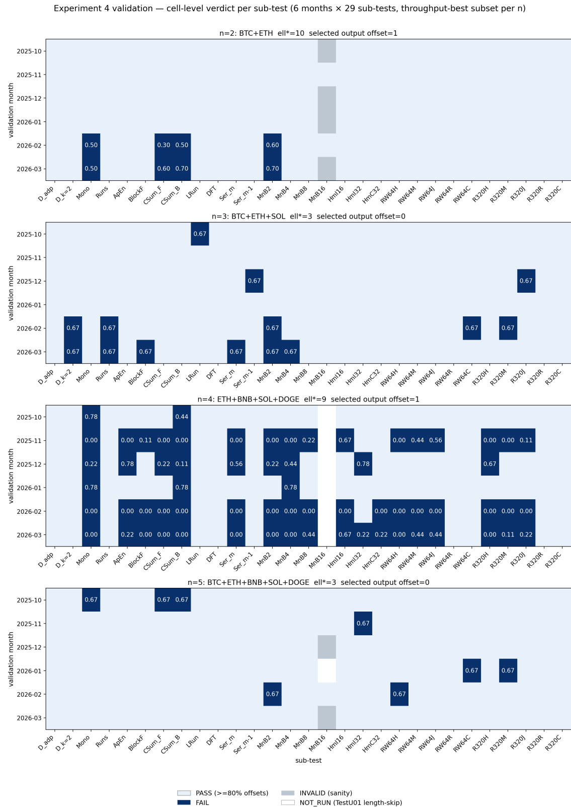
Figure 4.12: Experiment 4 – validation verdict matrix.
